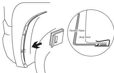
LEVER CLIP + SCREW W/WASHER
